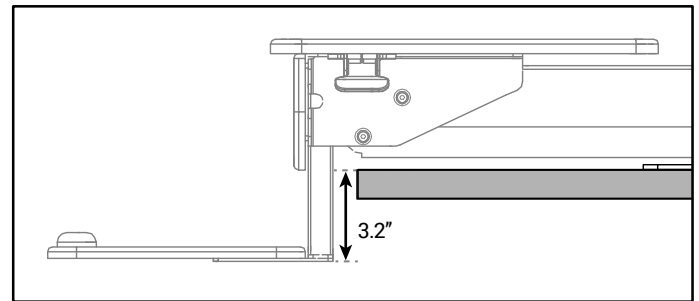
In the lowest position, keyboard tray hangs 3.2" below desktop surface with the long connector.
