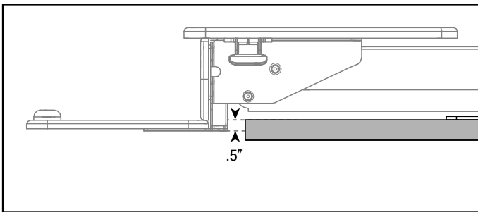
In the lowest position, keyboard tray hangs .5" below desktop surface with the short connector.
